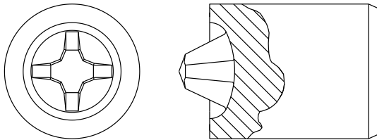
Pan Head Double Radius
