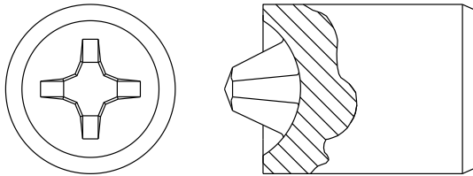
Pan Head
